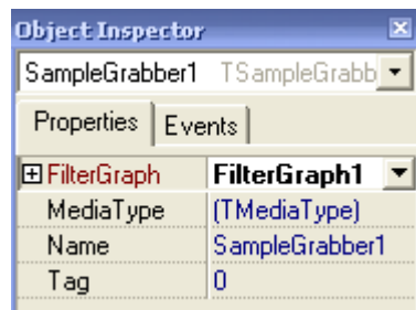
Gambar 5. Setting SampleGrabber
