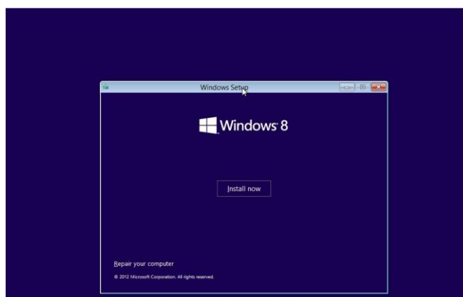
Install
