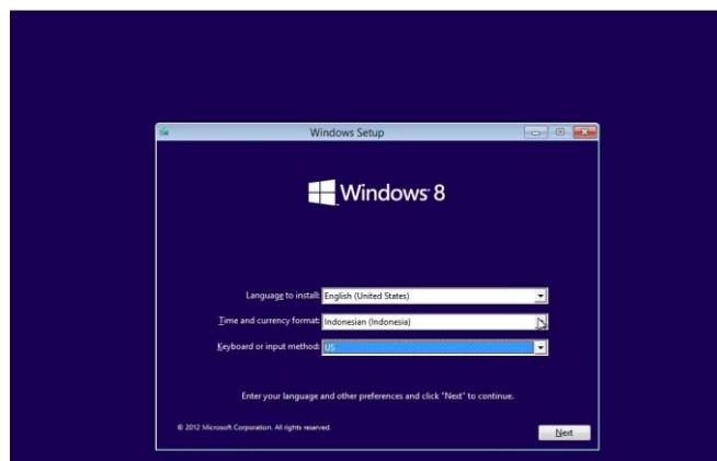
Windows Setup
