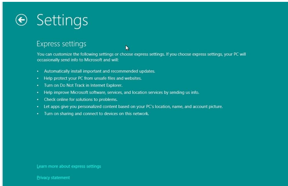
Express Settings
