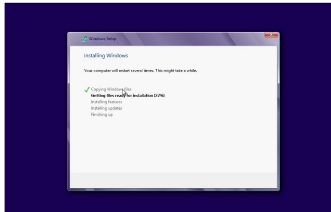
Proses Instalasi
