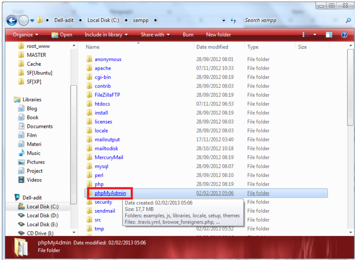
Gambar 2.2 Folder xampp
